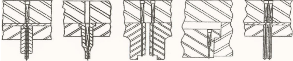
NARROW PUNCH IN SPLIT QUILL
